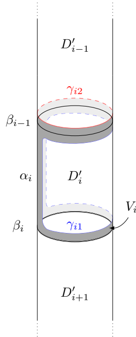
FIGURE 1. The annulus \mathcal{A} near D'_i .
