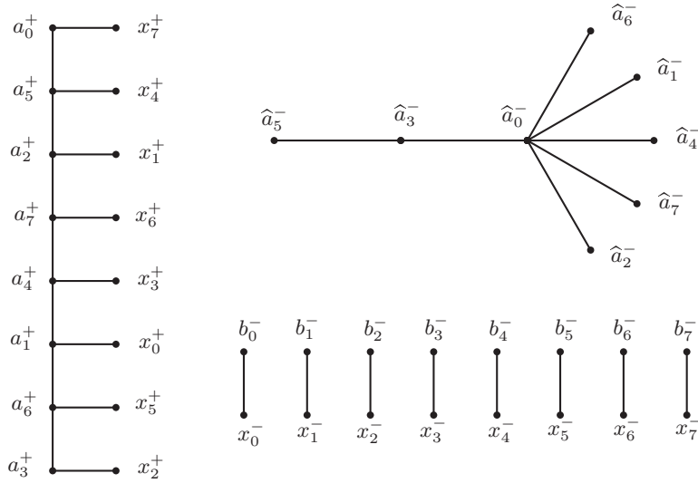
FIGURE 14. Ascending and descending links of v_2 in X .
