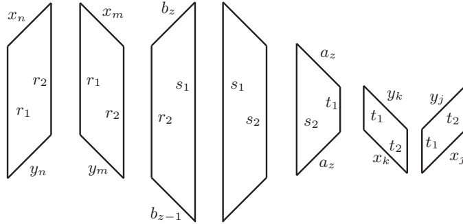
FIGURE 12. The Morse function \widehat{f} on the new 2-cells of C(X) .
