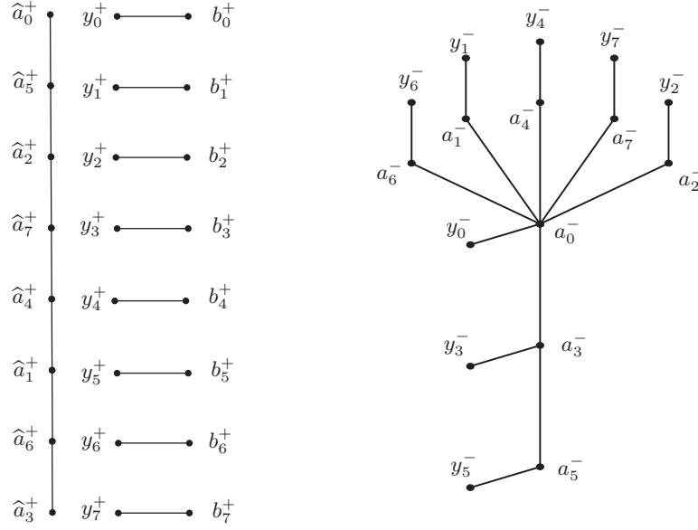
FIGURE 13. Descending and ascending links of v_1 in X .
