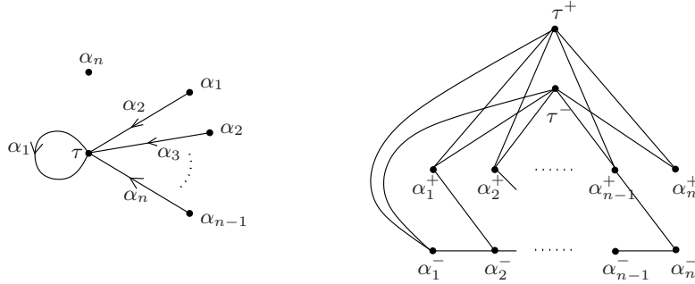
FIGURE 3. LOG presentation of F_n \rtimes_{\varphi} \mathbb{Z} , and link of vertex in associated squared 2-complex.
