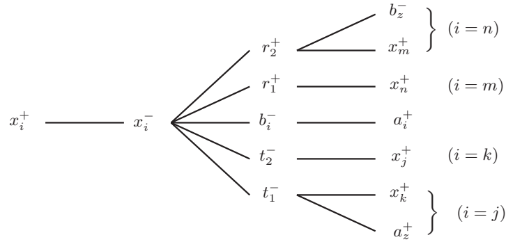
FIGURE 16. Finding a circuit around a vertex in P .
