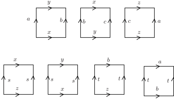
FIGURE 1. Hyperbolic free-by- \mathbb{Z} group with linearly distorted genus 2 surface subgroup.
