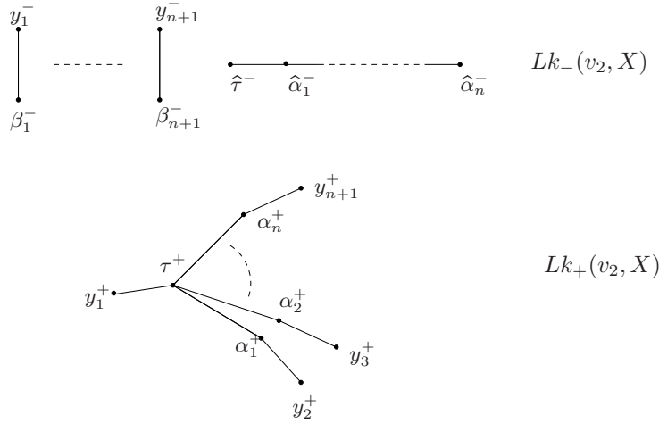
FIGURE 6. Ascending and descending links of v_2 in X .
