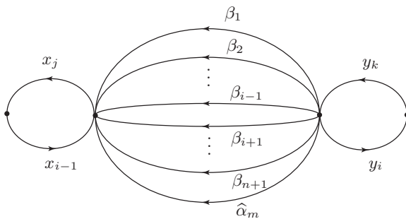
FIGURE 7. The graph \Gamma in the application of Theorem 1.8.
