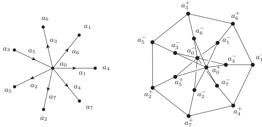
FIGURE 8. LOT presentation and link of vertex in presentation 2-complex.
