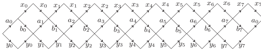
FIGURE 9. The non-positively curved, squared surface \Sigma .
