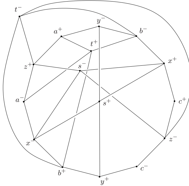
FIGURE 2. Link of the sole vertex v \in C(X) .
