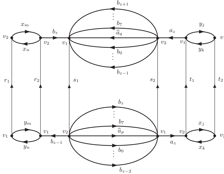
FIGURE 11. The complex \Gamma \times [0, 1] .
