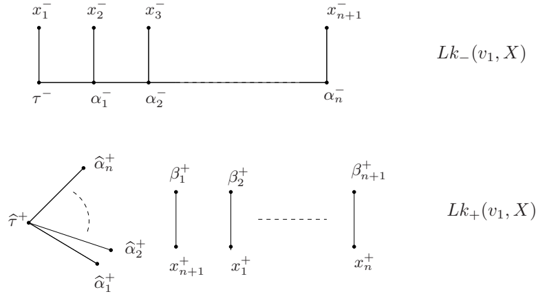
FIGURE 5. Ascending and descending links of v_1 in X .
