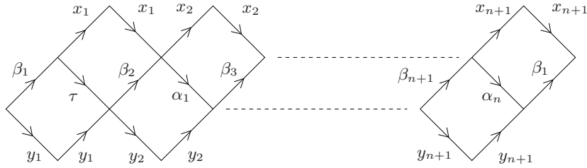
FIGURE 4. The non-positively curved, squared surface \Sigma_n .
