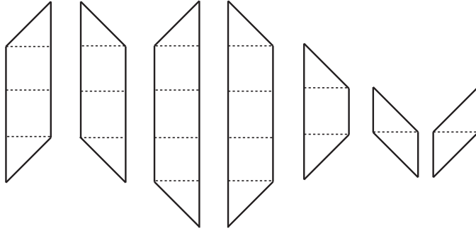
FIGURE 17. Circle vertex preimages in the 2-cells of \Gamma \times [0, 1] (cf. Figure 12).
