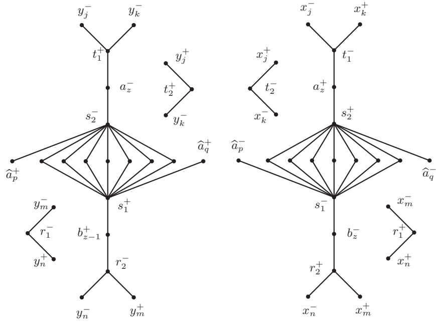
FIGURE 15. The portions of Lk(v_1, C(X)) and Lk(v_2, C(X)) contributed to by \Gamma \times [0, 1] .
