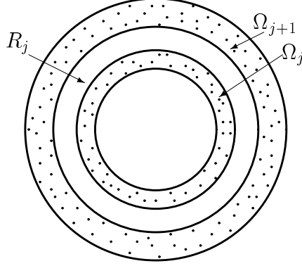
FIGURE 2. The j -inclusion: two consecutive \Omega -regions ( \Omega_j and \Omega_{j+1} ) filled in with scattered dots that do not overlap. The white region in between is defined as R_j .
