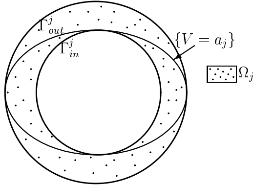
FIGURE 1. Formation of a region \Omega_j . \Gamma_{out}^j ( \Gamma_{in}^j ) is the outmost (inmost) tangency of an orbit of Z with \{V = a_j\} (symbolized here by an ellipse). \Omega_j is the region filled in with scattered dots.
