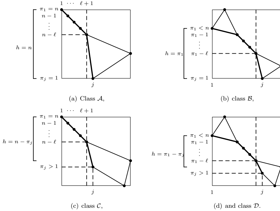
FIGURE 4. The four subclasses of square polygons (cases of a non-empty initial sequence of double points).
